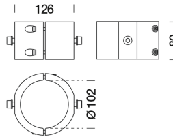
8951045 Connection to the pole 102 mm Ø
