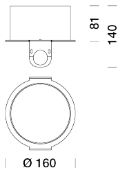
8935601 Cylindrical screen
