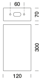
8950110 Extension base H. 300 mm (TARGET Medium version)
