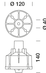
8945039 Recessed box IP67 H. 160 mm with base \varnothing 120 mm
