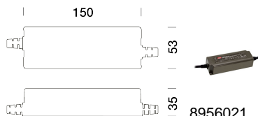
8956021 Power supply DALI (24V DC - 60W) IP67
