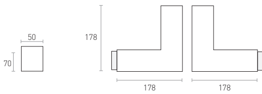
UNIÓN LED EN L LED L JOINT
