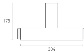
UNIÓN LED EN T LED T JOINT
